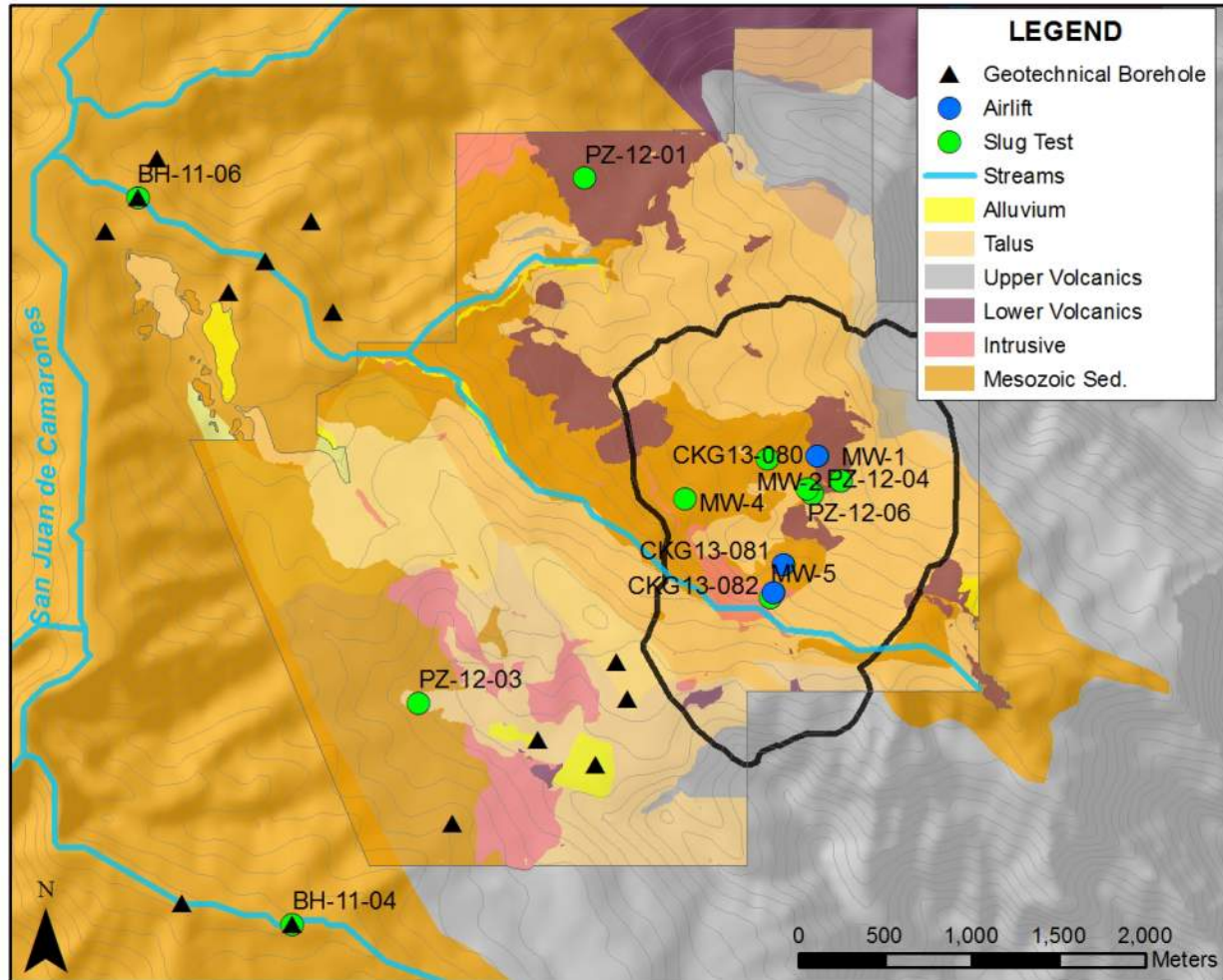
Figure 20-7: Borehole Locations of Airlift and Slug Tests
