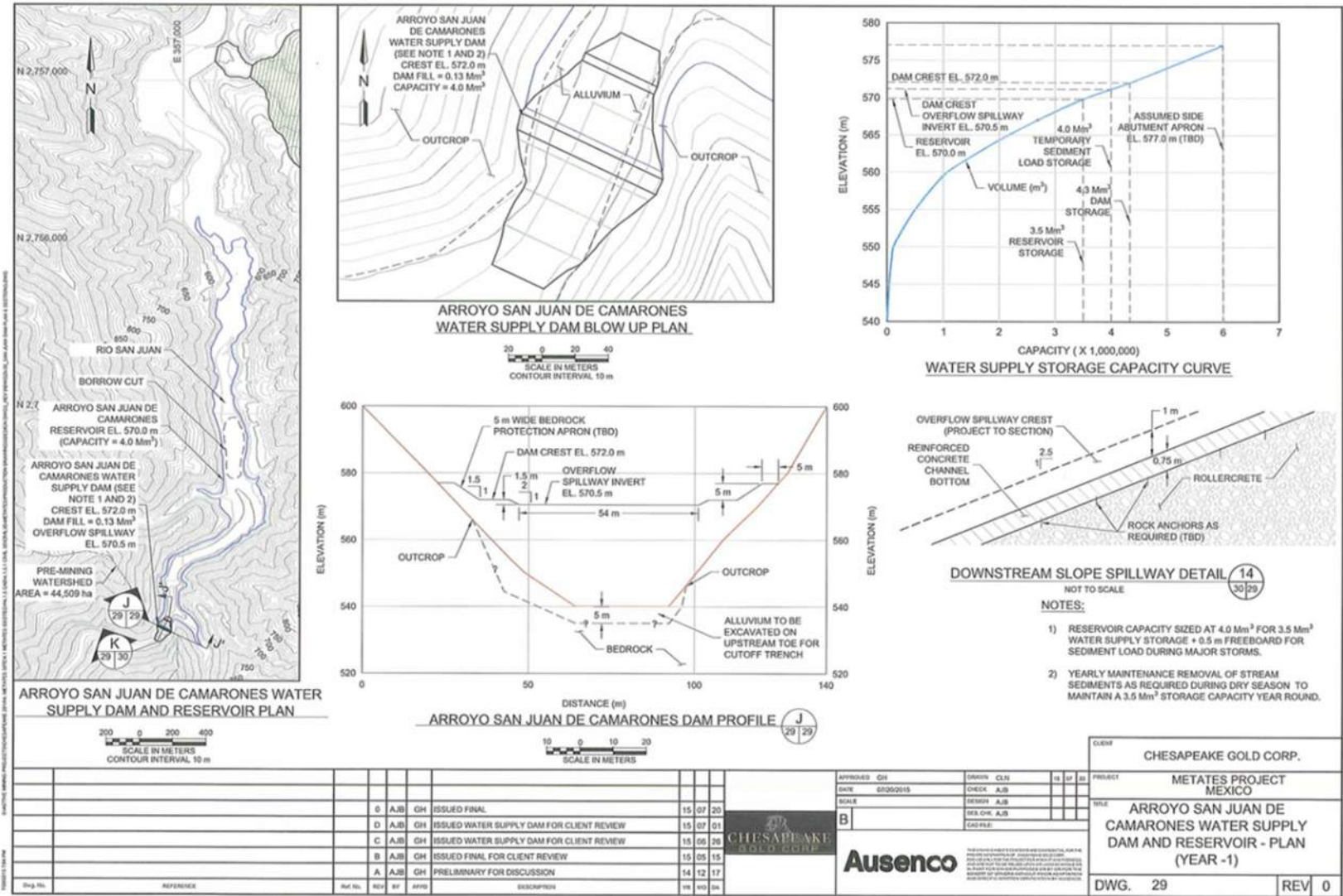
Figure 18-3: San Juan de Camarones Dam and Reservoir Plan and Sections
