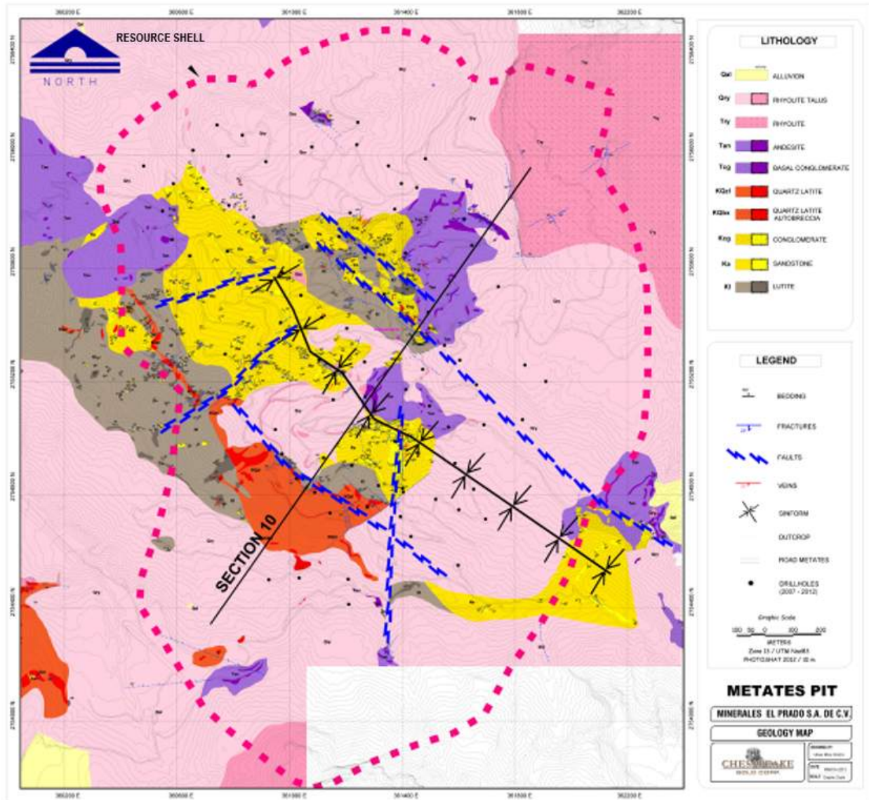
Figure 7-3: Geology of the Metates Pit Area, Chesapeake 2016
