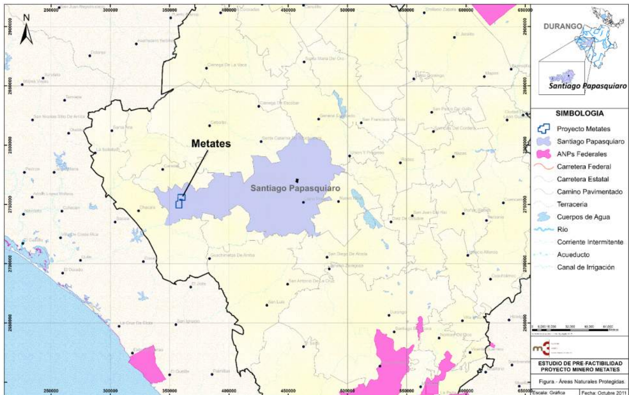
Figure 20-4: Natural Protected Areas (ANP Federales)
