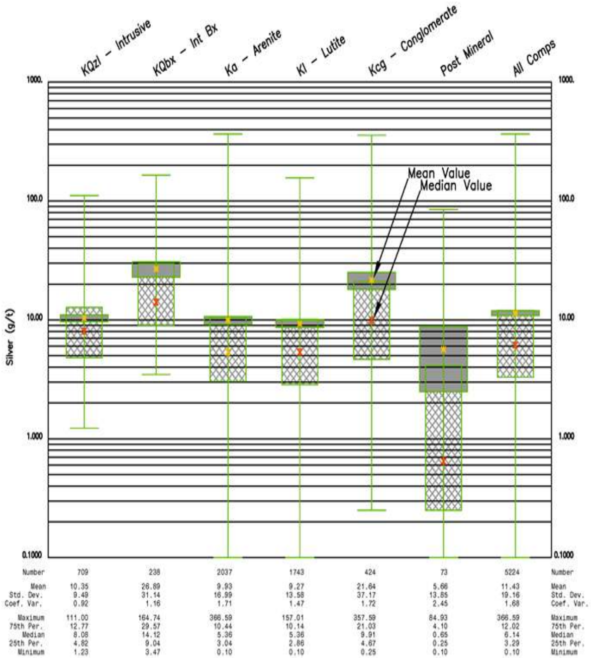
Silver Grades in 15m Composites by Lithology Type Light Gray Box Shows 25%, 75% and Median, Dark Gray Shows Mean and 95% Conf Interval Figure 14-4: Silver Grades in 15 m Composites by Model Lithology Type, IMC 2016
