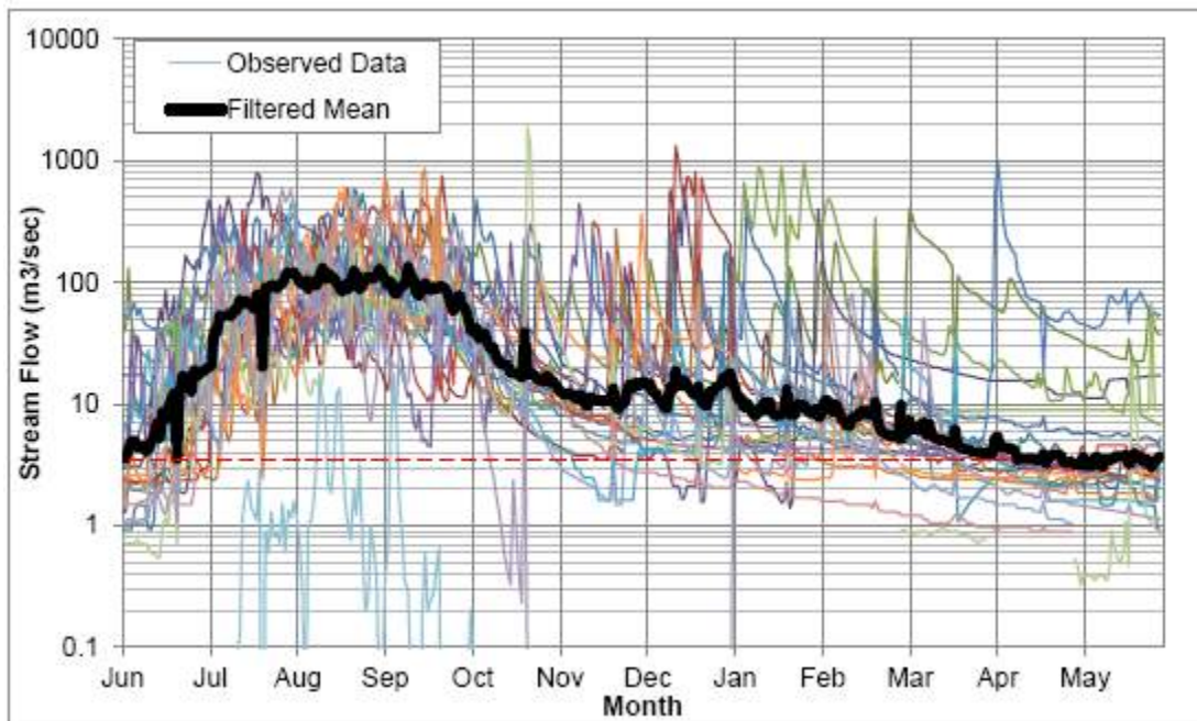
Figure 20-3: Streamflow of San Lorenzo River at EI Real
