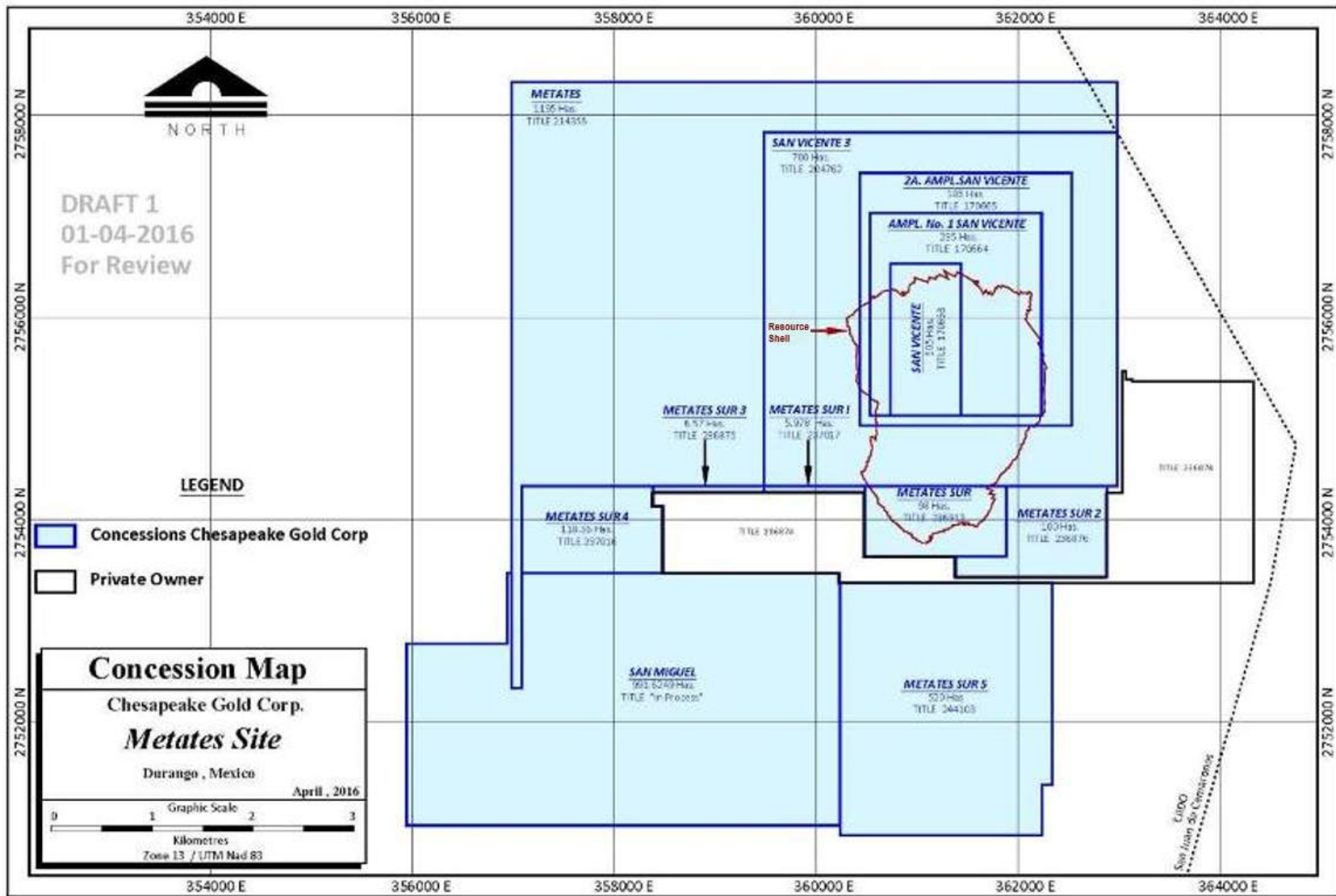
Figure 4-2: Mining Concessions in the Metates Area
