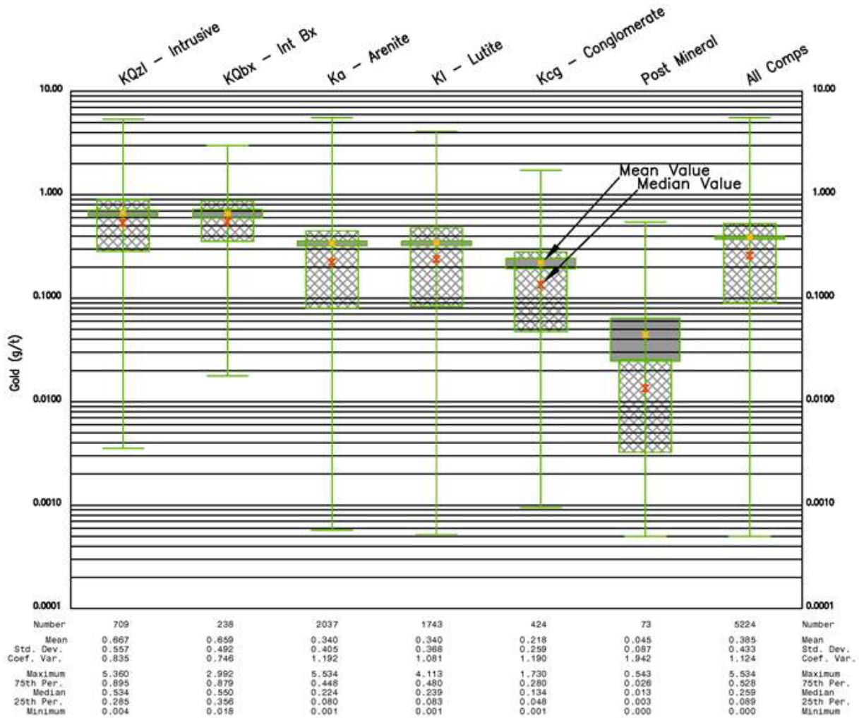
Gold Grades in 15m Composites by Lithology Type Light Gray Box Shows 25%, 75% and Median, Dark Gray Shows Mean and 95% Conf Interval
