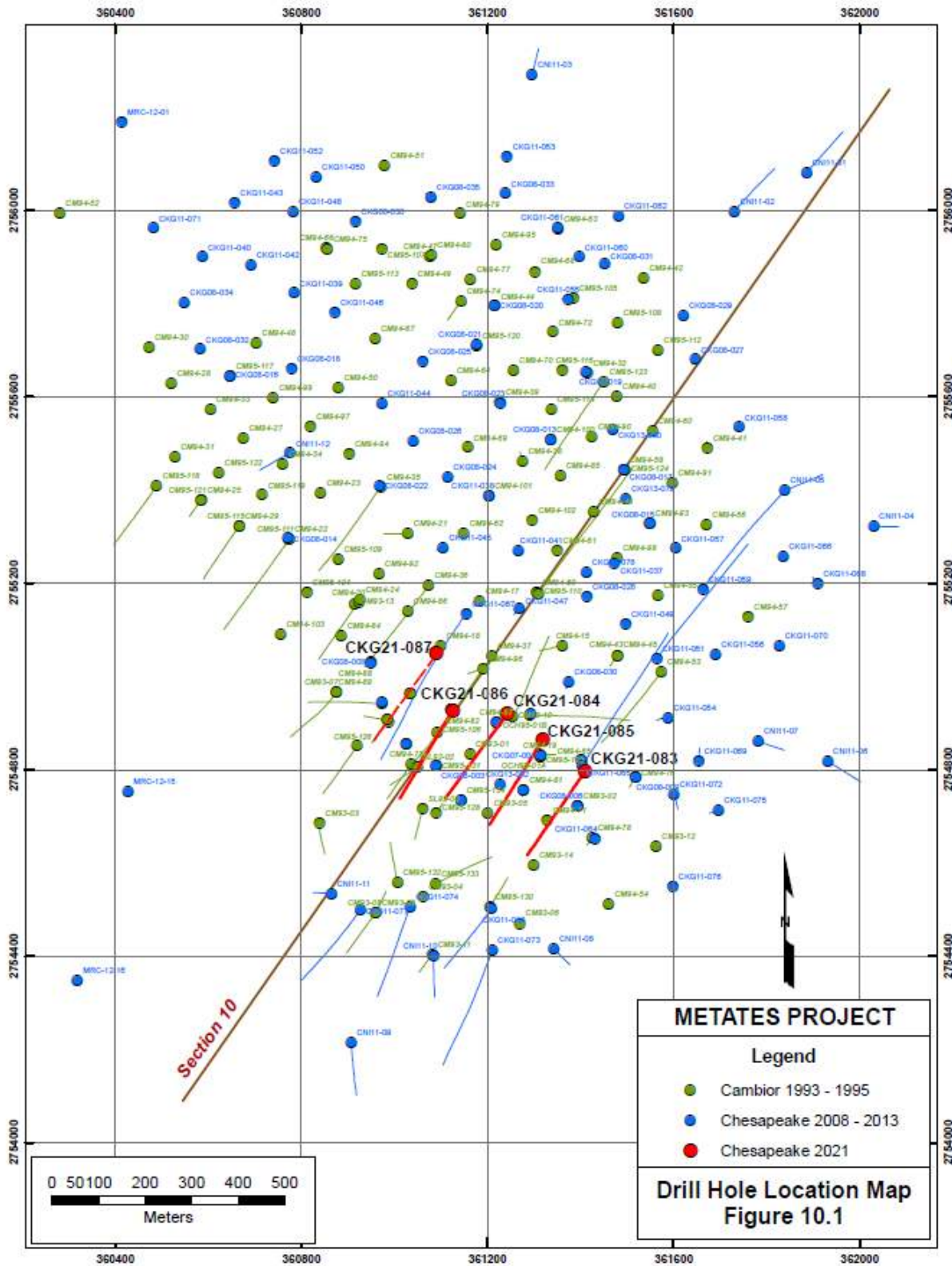
Figure 10-1: Drillhole Locations, Chesapeake 2021
