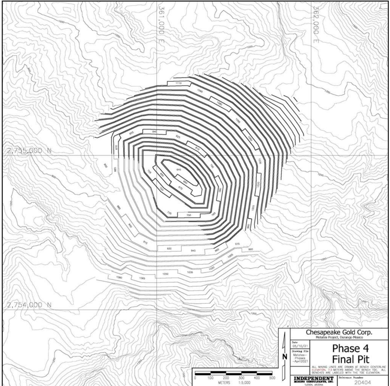
Figure 16-5: Metates Final Pit (Phase 4), IMC 2021
