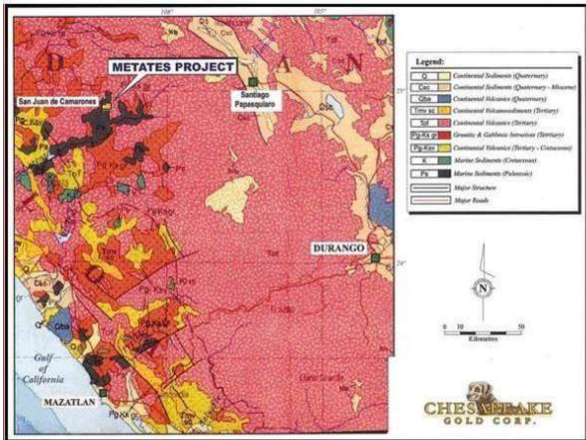
Figure 7-1: Regional Geology, Chesapeake 2016
