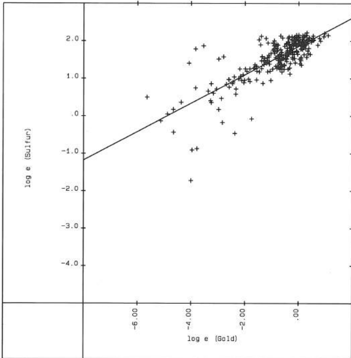
Figure 14-9: Gold vs. Sulphur – Intrusive Rock Types, IMC 2016
