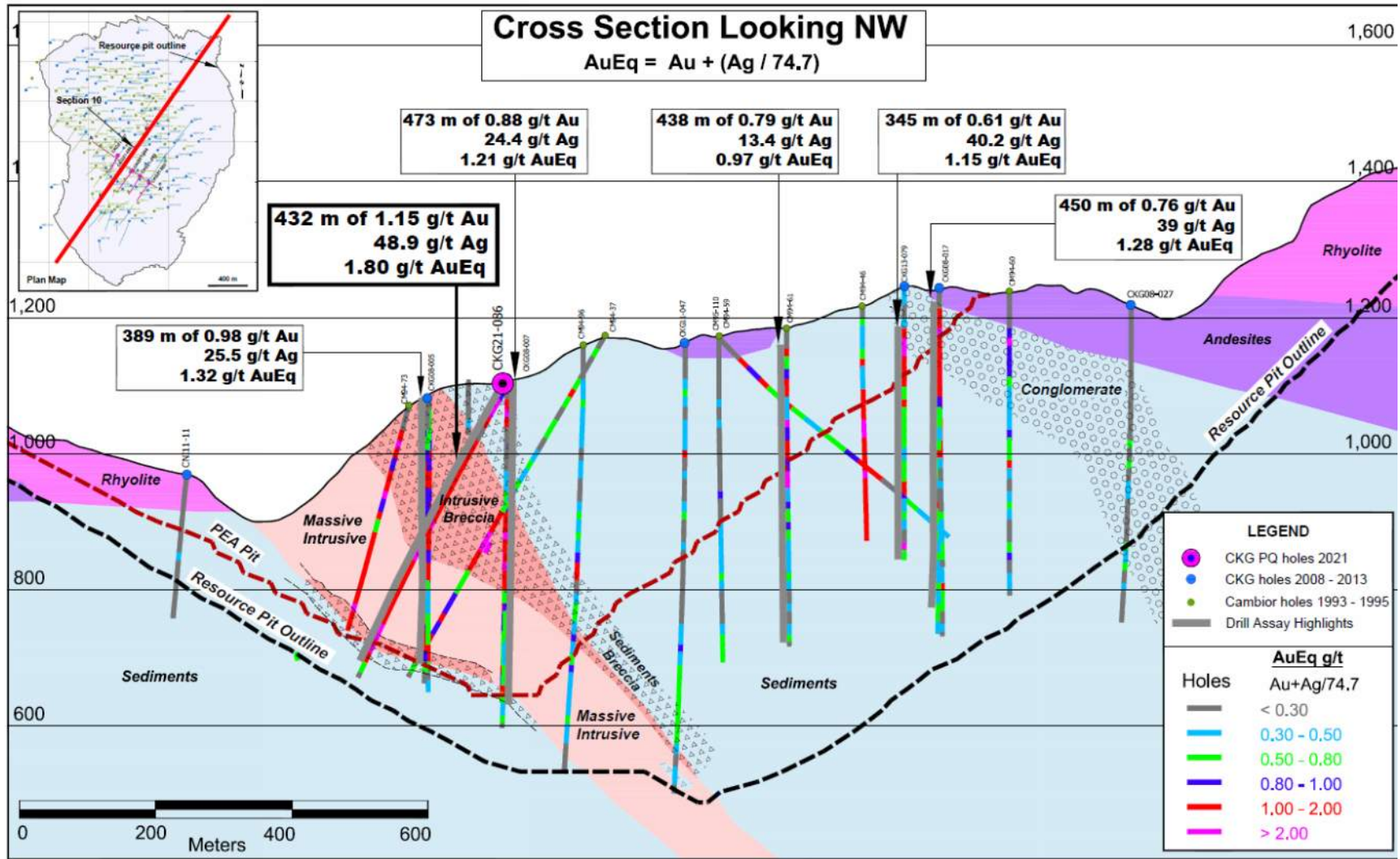
Figure 7-4: Geology and Mineralization on Cross Section 10,300E, Chesapeake 2021
