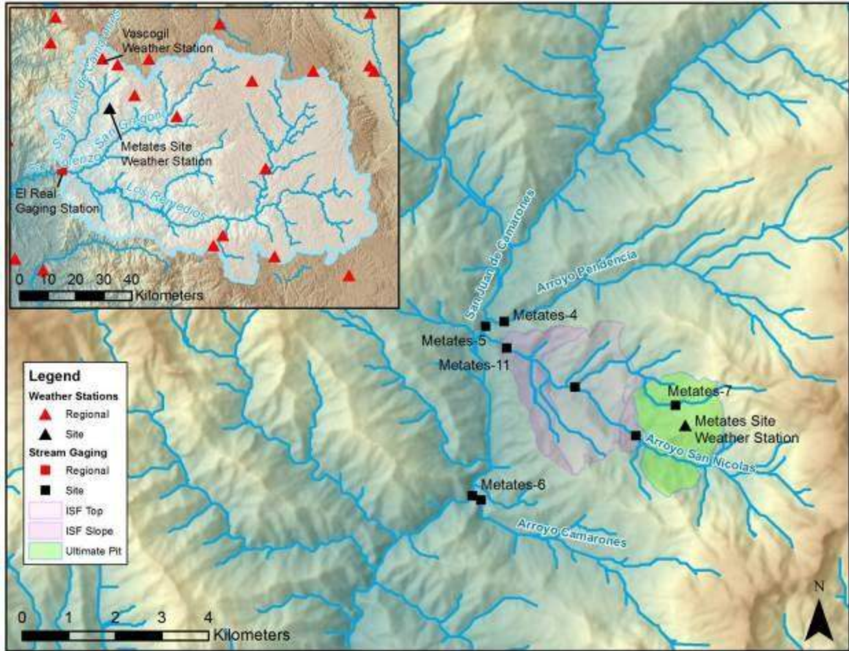
Figure 20-1: San Lorenzo River Watershed Above El Real
