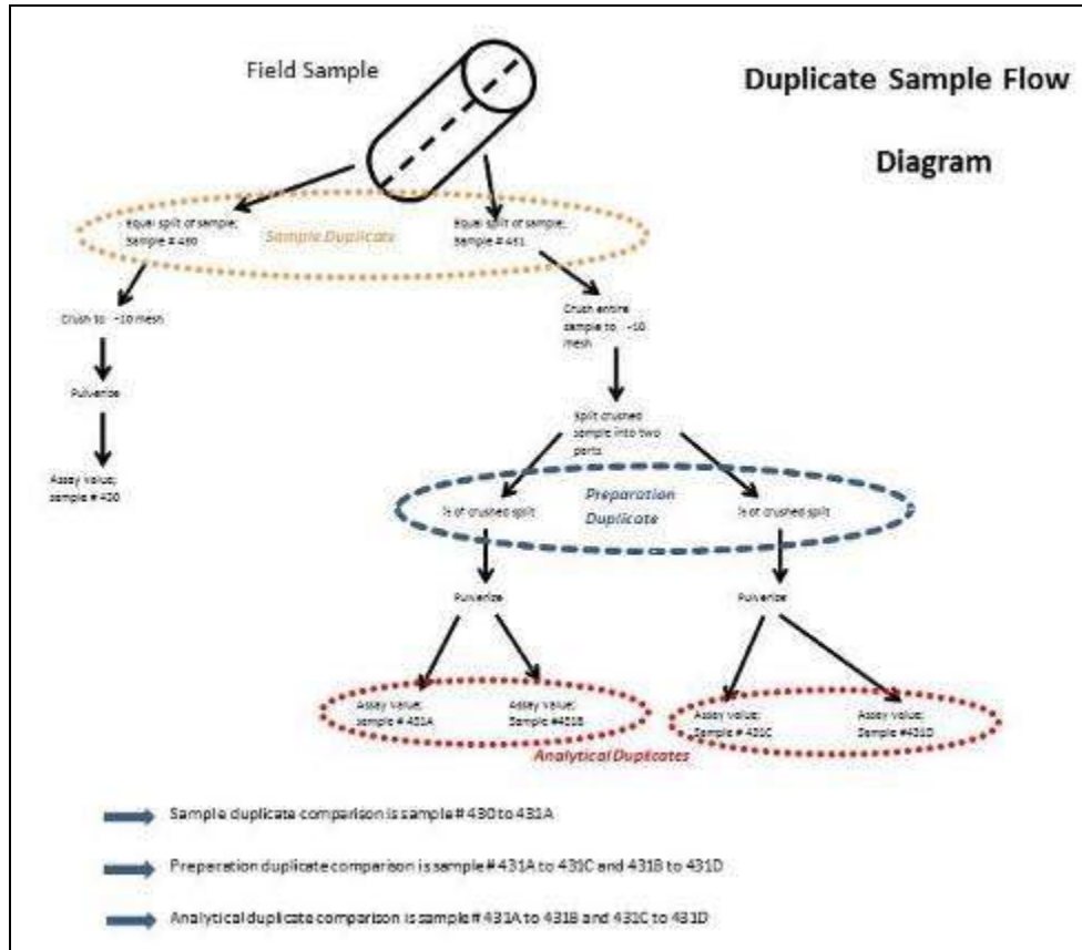
Figure 11-1: Duplicates Sampling Scheme, GAI 2009
