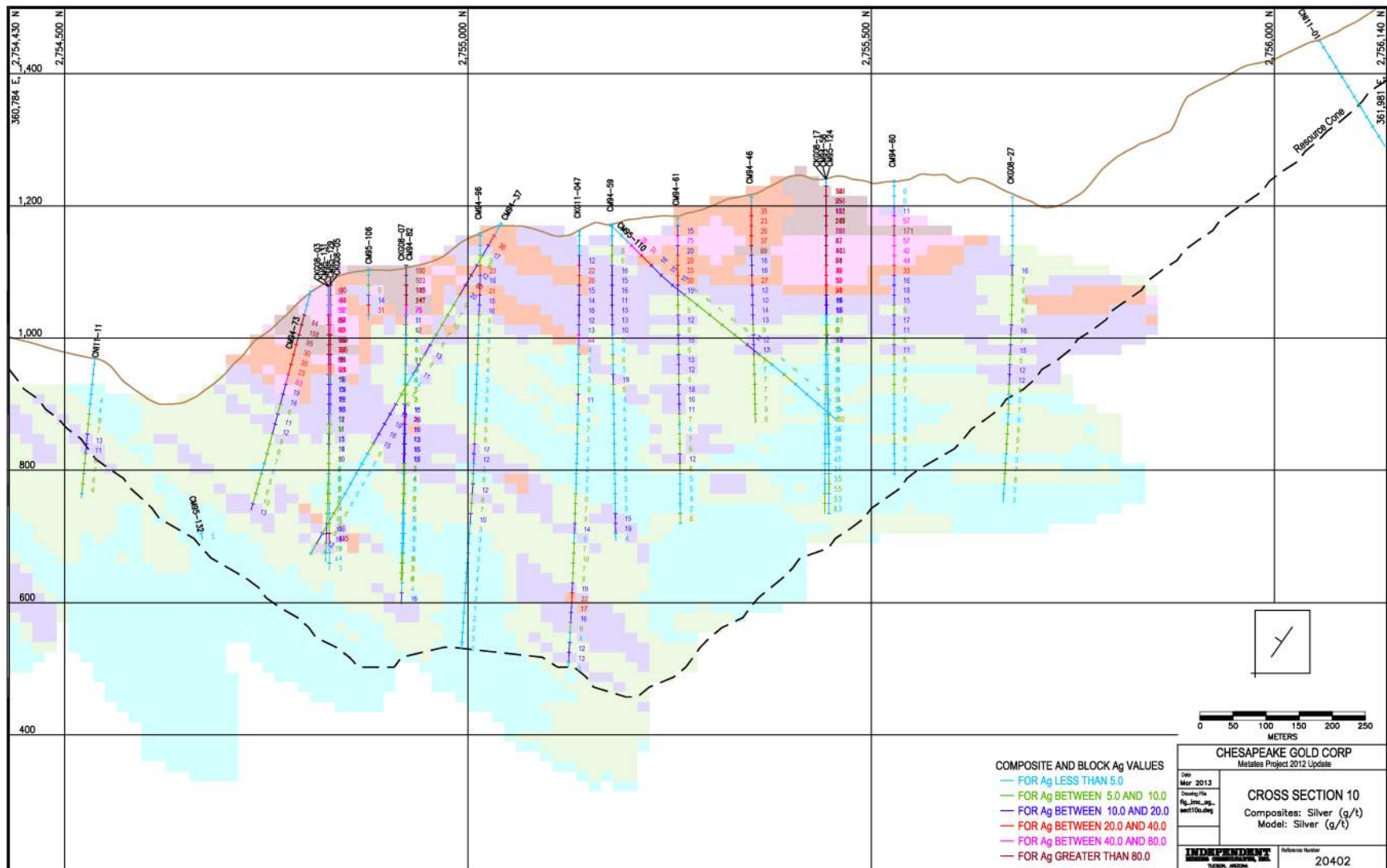
Figure 10-3: Silver Grades on IMC Section 10, IMC 2014
