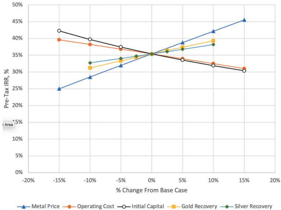
Figure 25-2: Sensitivity of IRR to Metal Prices, Operating Cost, Capital Cost and Metal Recoveries
