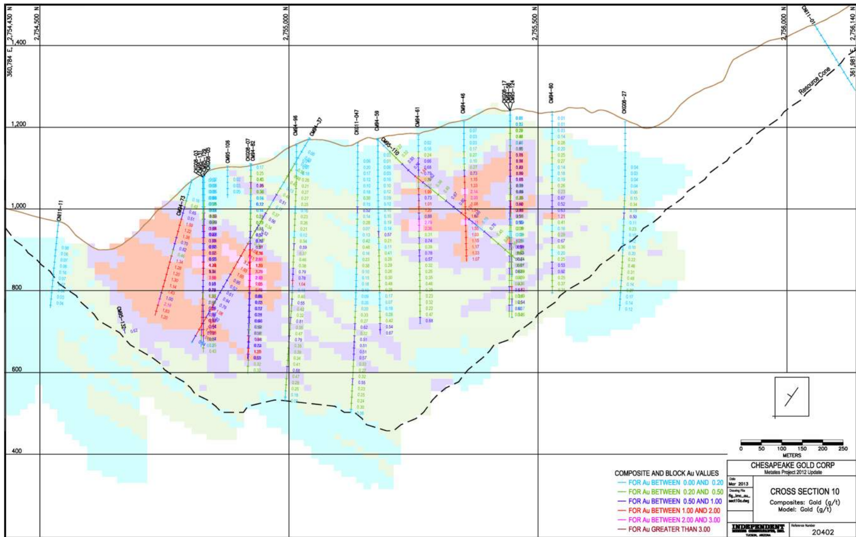
Figure 10-2: Gold Grades on IMC Section 10, IMC 2014
