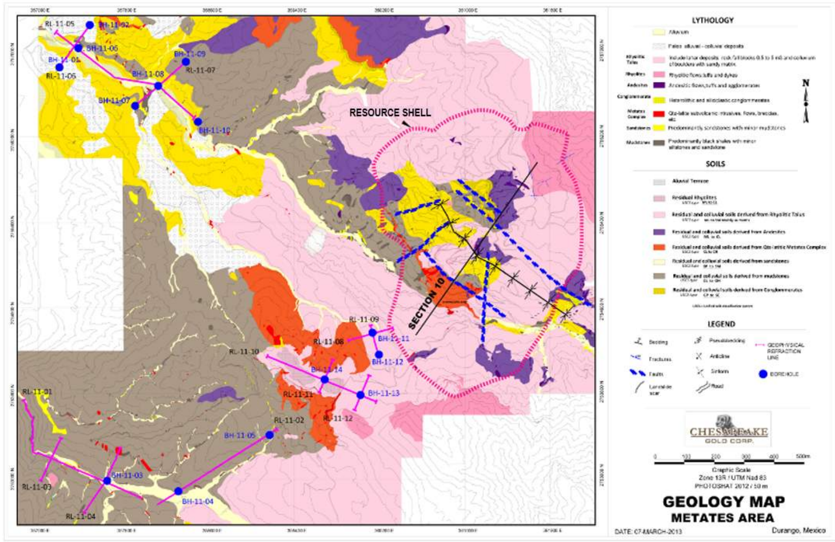
Figure 7-2: Geology of the Metates Area, Chesapeake 2016
