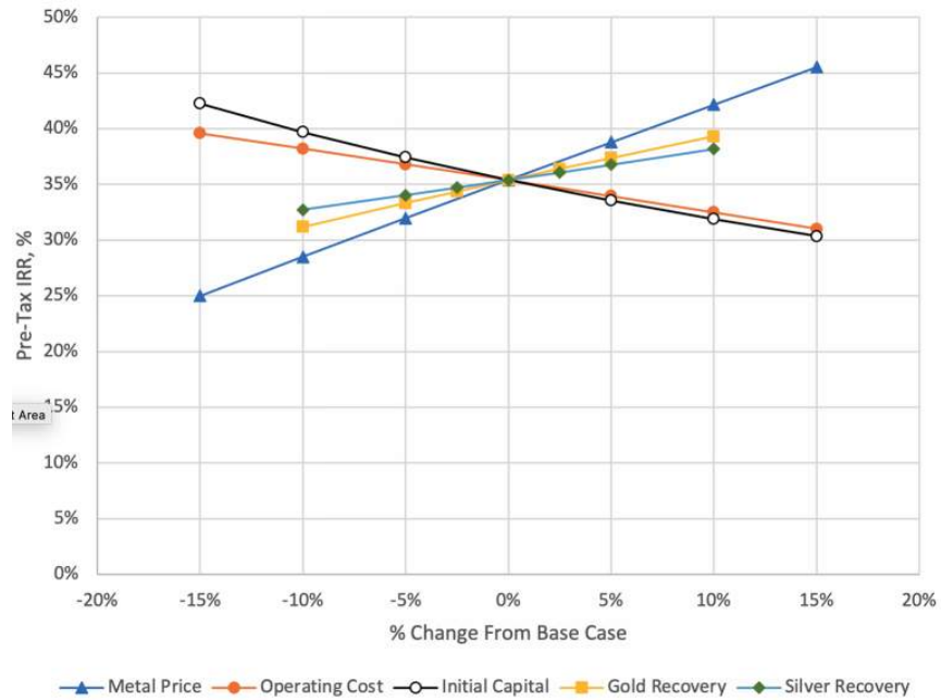
Figure 1-7: Sensitivity of Pre-Tax IRR to Metal Prices, Operating Cost, Capital Cost and Recovery
