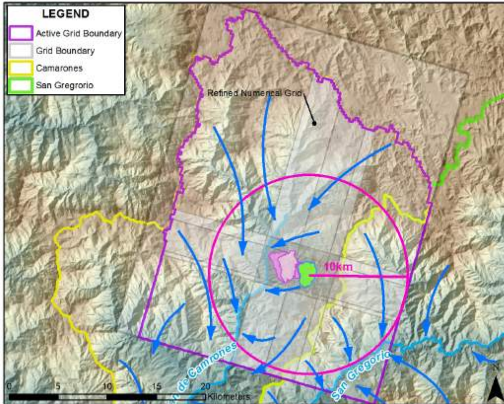
Figure 20-8: Numerical Model Active Grid Area
