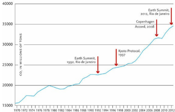
Global CO 2 Emissions, 1970–2013
