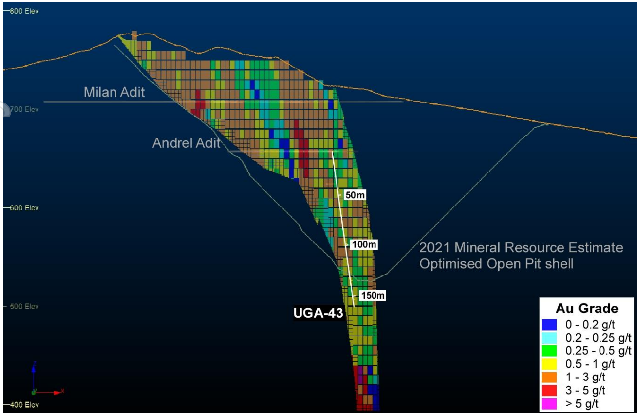
Figure 2: Cross-section through the existing Sturec Mineral Resource displayed as a Mineral Resource blocks, which are 10m high and 5m wide (Au grade scale shown with pseudocolor spectrum). This view is looking north.
