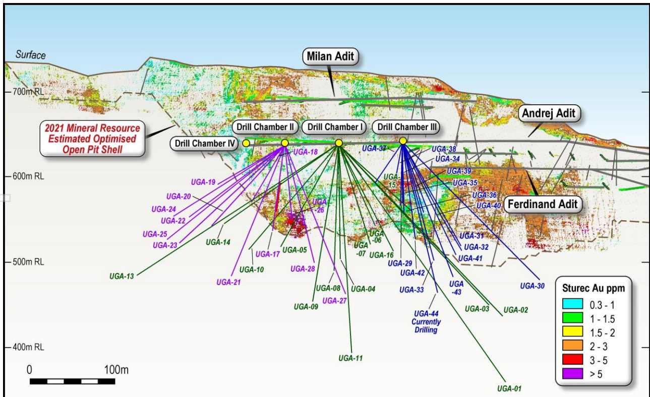
Figure 1: Long-section showing the traces of drill holes from the various drill chambers; shown relative to mineralisation within the existing Sturec Mineral Resource displayed as a 3D point cloud (grade scale shown with pseudocolor spectrum). This view is looking west
